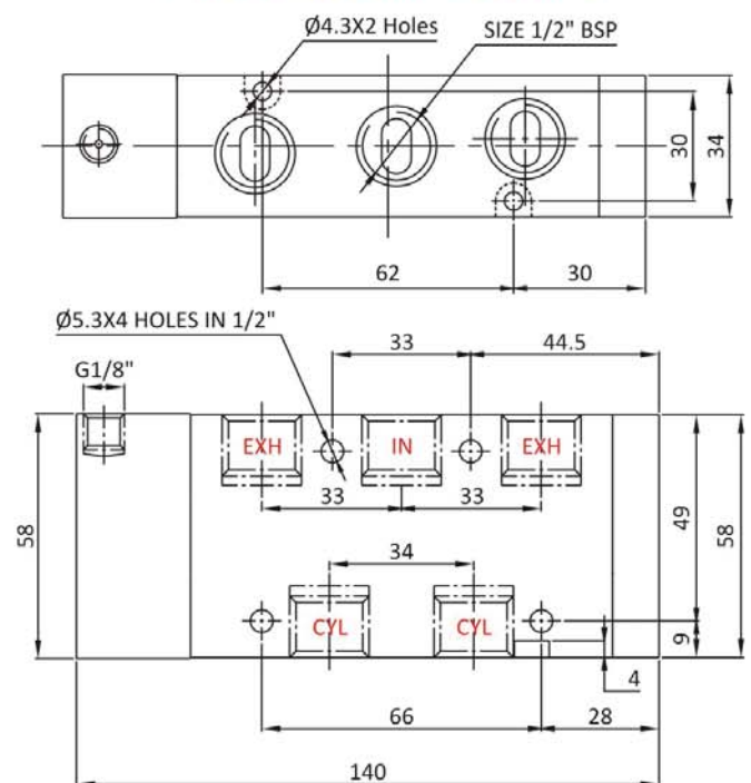
Size : 1/2" BSP (Dimensions are in mm)
